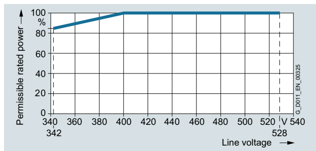
Permissible rated power as a function of the line voltage for PM230 Power Modules, frame sizes FSA to FSF
