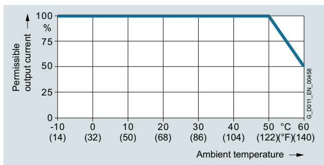
Permissible output current as a function of the ambient temperature for high overload (HO) PM230 Power Modules, frame sizes FSA to FSC
