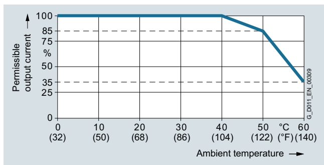
Permissible output current as a function of the ambient temperature for low overload (LO) for PM230 Power Modules, frame sizes FSD to FSF
