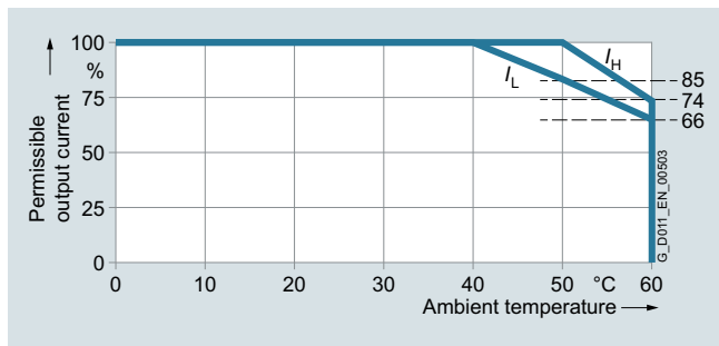
Permissible output current as a function of the ambient temperature for low overload (LO) and high overload (HO)
