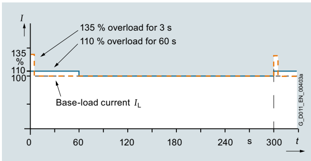
Overload capability, low overload for SINAMICS G120P Cabinet from 160 kW (215 hp)
