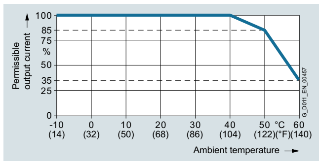
Permissible output current as a function of the ambient temperature for low overload (LO) for PM230 Power Modules, frame sizes FSA to FSC
