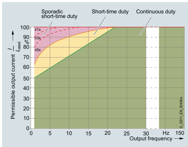
Overload capability, high overload
