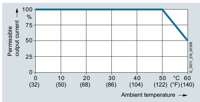
Permissible output current as a function of the ambient temperature for high overload (HO) PM230 Power Modules, frame sizes FSD to FSF
