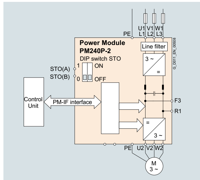
Connection diagram for PM240P-2 Power Module with or without integrated line filter class A
