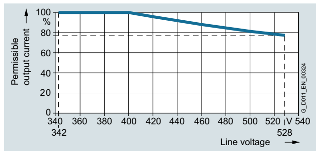
Permissible output current as a function of the line voltage for PM230 Power Modules, frame sizes FSA to FSF
