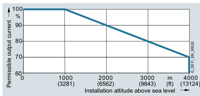
Permissible output current as a function of the installation altitude for PM230 Power Modules, frame sizes FSA to FSF
